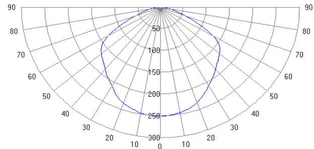
Polar Candela Distribution Plot Using Missed Rays
